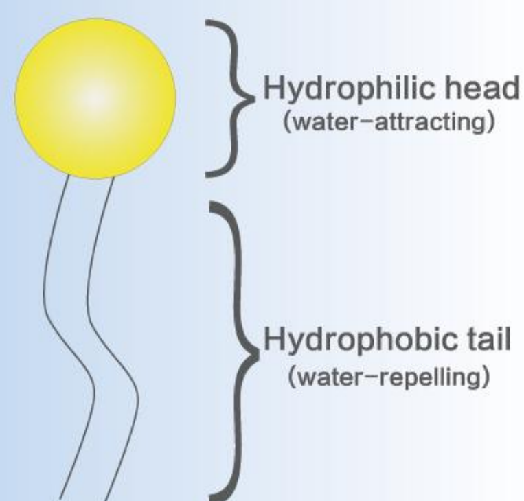
simplified structure of phospholipid
